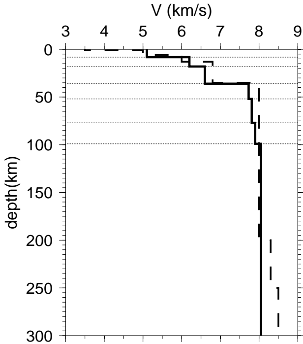
Fig. 4. P-wave velocity models for Costa Rica. 1D-models used for routine earthquake location by OVSICORI-UNA (solid line) and RSN (broken line).
